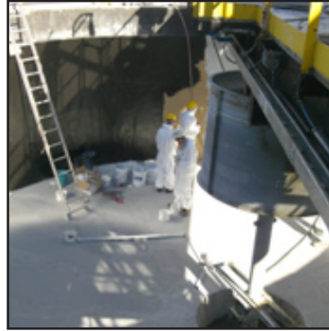
Application of Belzona® 5811
