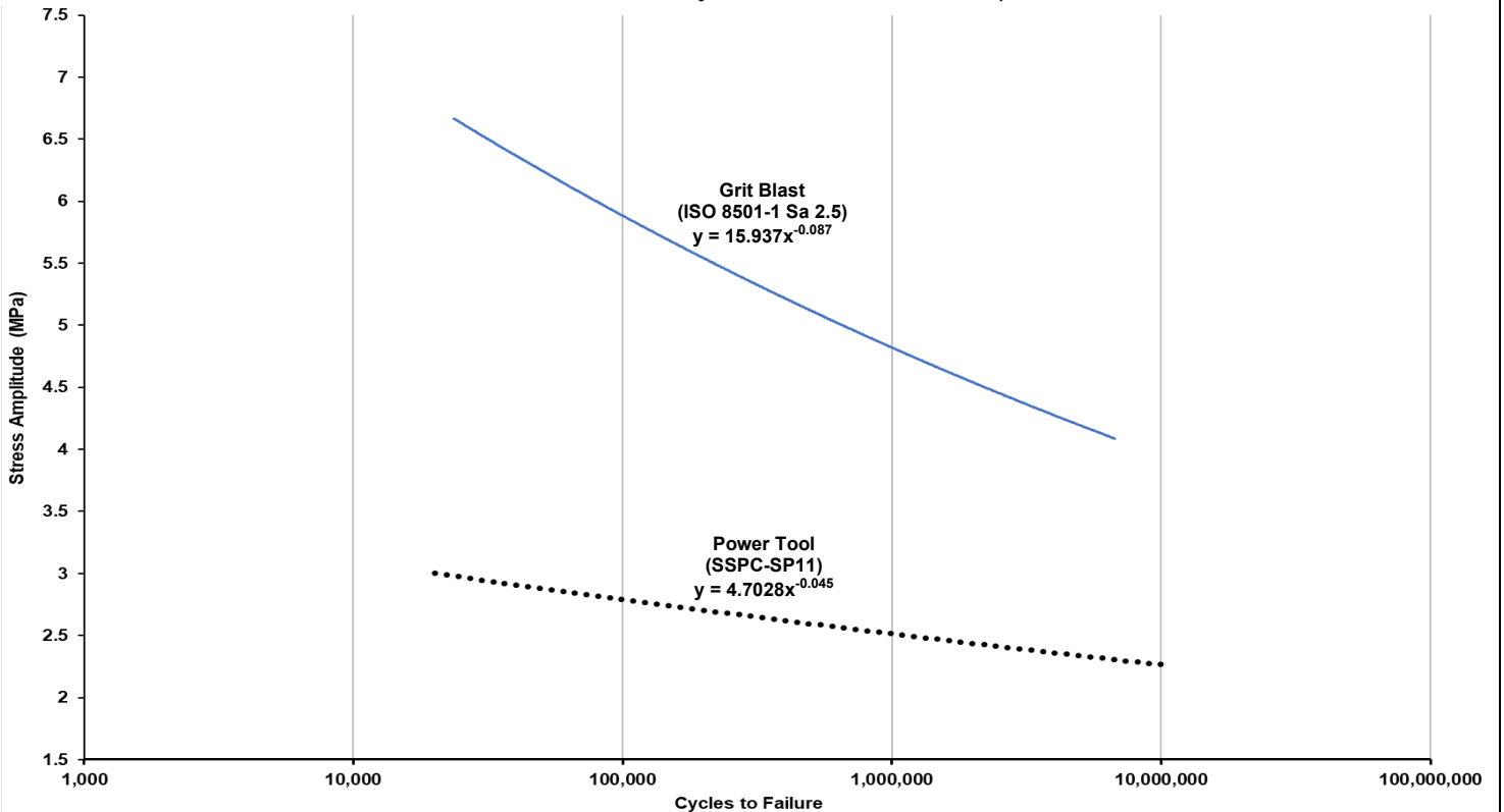
ISO 9664 - Belzona 7311 Cycles to Failure vs. Stress Amplitude
