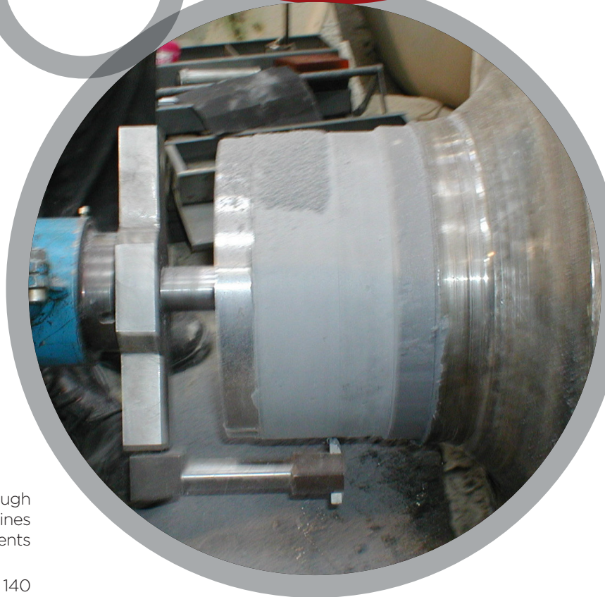
Shaft Rebuilding
