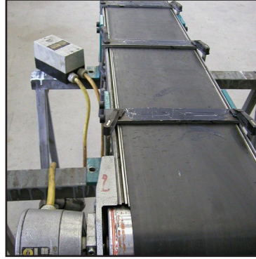
Steel plates moulding Elastomer to shape
