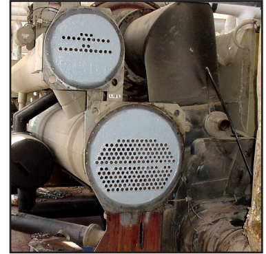
Tube sheets were protected by Belzona® 1321
