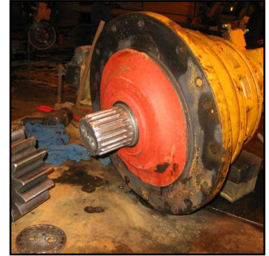
Worn gear and drive
