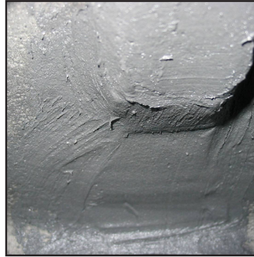
Rebuilding cavitation area using Belzona® 1311 (Ceramic R-Metal)
