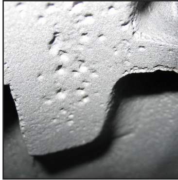
Cavitation area after blasting
